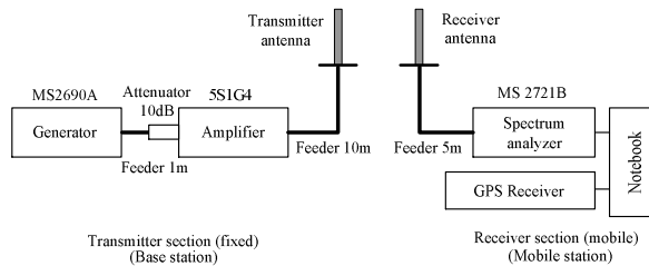
Fig. 3. Block diagram of measuring equipment set.
