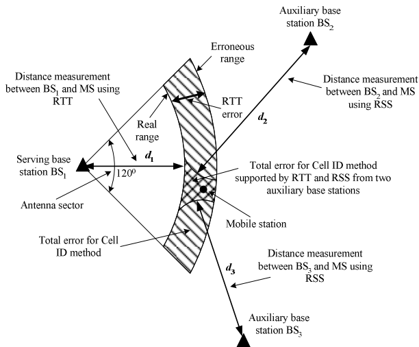
Fig. 1. Cell ID method supported by RSS.
